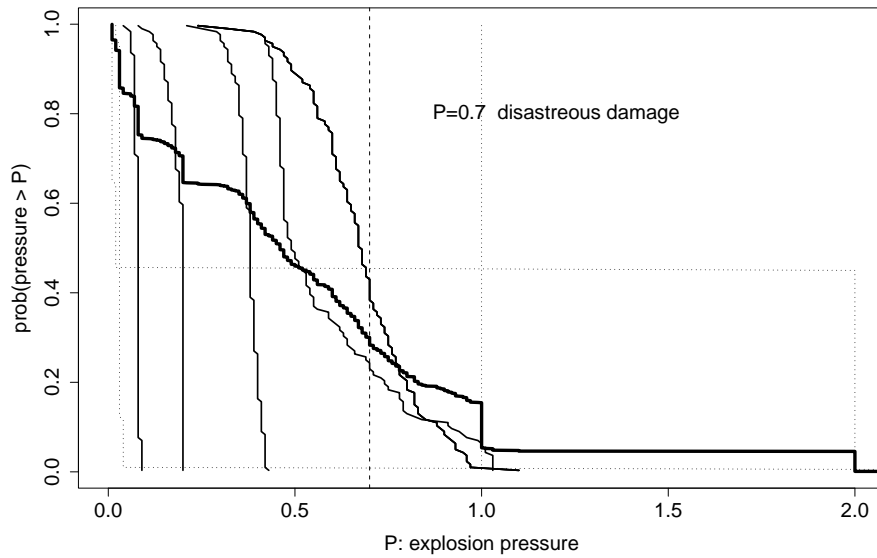
Figure 3: Distribution of pressure ccdf s conditional to initial intensity I .
